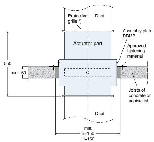
Option 2 Joist system
